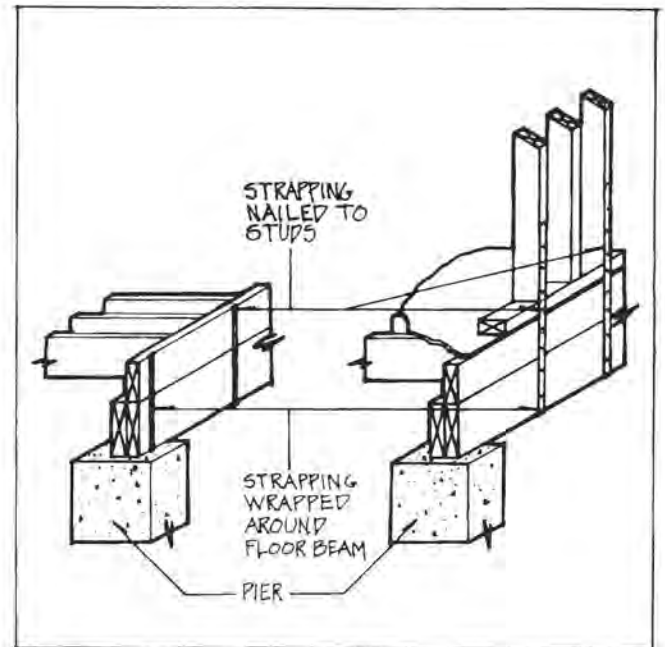
Figure 4.43. Metal Strapping
