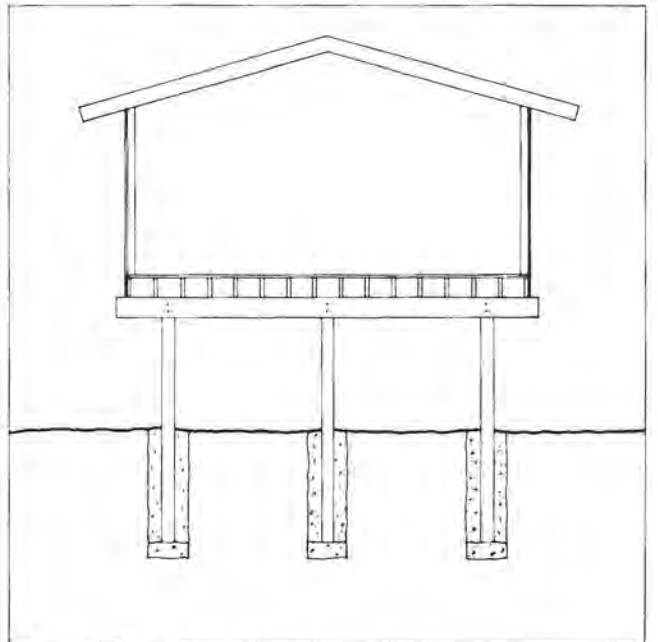
Figure 4.28. Platform Construction
