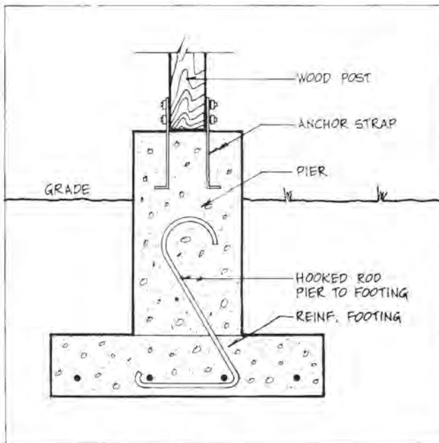
Figure 4.9. Post/Pier Foundation
