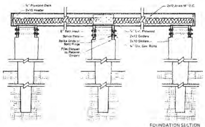
FOUNDATION SECTION
