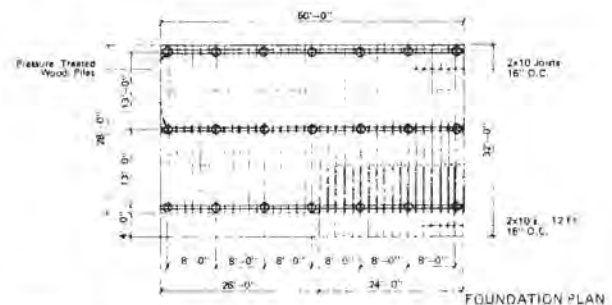
FOUNDATION PLAN
