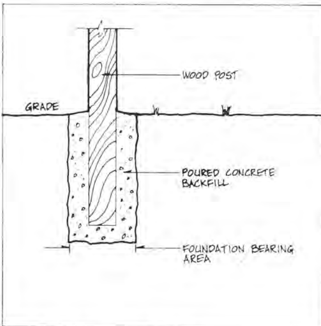
Figure 4.10. Concrete Backfill
