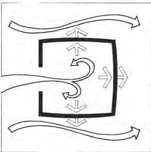
Figure 2.4. Wind Forces
