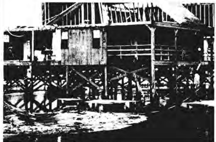
Figure 4.23. Diagonal Bracing
